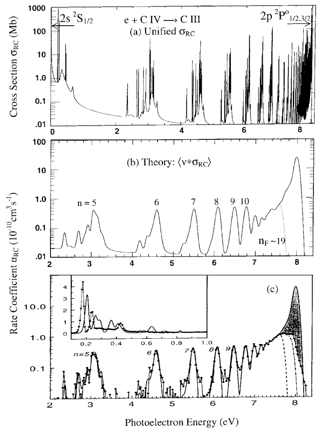
FIG. 1. (a) Unified ( e + \text{C IV} ) recombination cross section \sigma_{\text{RC}} with detailed resonance structures; (b) theoretical rate coefficient \langle \nu \cdot \sigma_{\text{RC}} \rangle convolved over a Gaussian with experimental FWHM [2]; (c) the experimentally measured rate coefficient [2]. The unified \sigma_{\text{RC}} in (a),(b) incorporate the background cross section eliminated from the experimental data in (c). The dashed and dot-dashed lines represent approximate field ionization cutoffs (see text).
