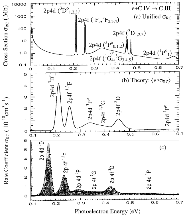
FIG. 2. (a) The 2p4l resonance complex, detailed unified \sigma_{RC} ; (b) convolved rate coefficient ( v \cdot \sigma_{RC} ); (c) experimentally measured values from CRYRING [1] (open circles), TSR [2] (solid circles), and theoretical calculations from [1] (shaded region). The solid circle in (b) at E = 0.1 eV represents the experimentally measured background values (Fig. 7 in [2]).
