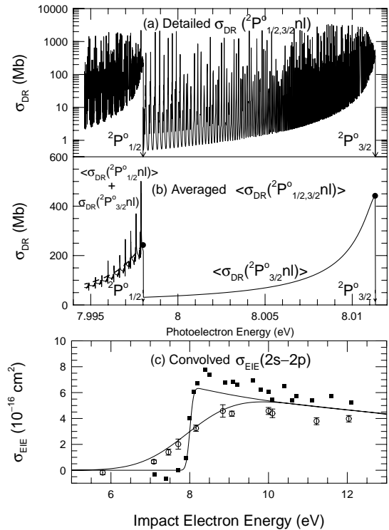
FIG. 3. \sigma_{DR} and \sigma_{EIE} of C IV: (a) detailed \sigma_{DR} with 2P_{1/2,3/2}^0 n\ell resonances; (b) \sigma_{DR} averaged over 2P_{1/2}^0 n\ell and detailed 2P_{3/2}^0 n\ell resonances (solid line), average over the 2P_{3/2}^0 n\ell (dashed line) (the solid circles are the peak averaged \sigma_{DR} ); (c) \sigma_{EIE} convolved over experimental data with FWHM = 0.175 eV from [16] (solid squares) and with FWHM = 2.3 eV from [17] (open circles).
