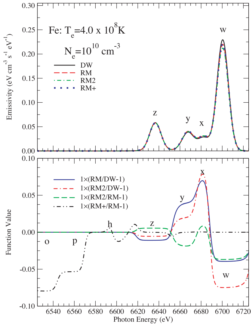
Figure 5. Top panel: calculated Fe spectra at T_e = 4.0 \times 10^8 K and N_e = 10^{10} \text{ cm}^{-3} for each of the Fe data sets. Bottom panel: functions of the spectra presented for comparison. Again, there is an excellent agreement between all spectra. The largest uncertainties are in very weak satellite lines, as well as the w and x lines.
