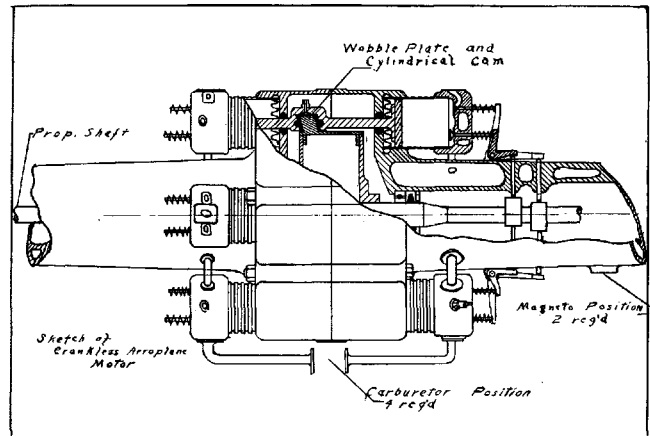
Sketch of the Crankless Motor
