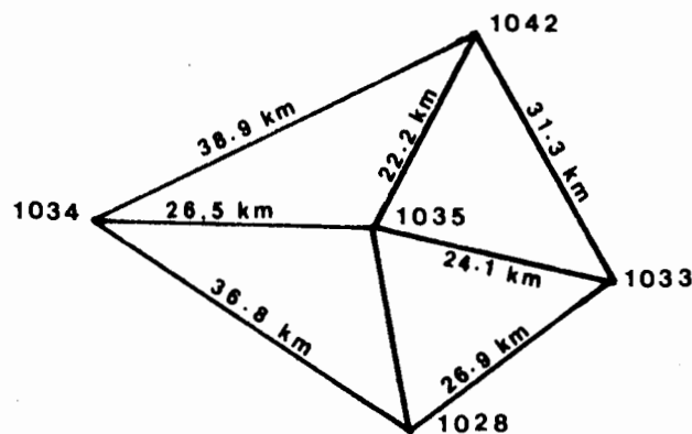
Figure 5-10 A Typical Five-Station Setup
