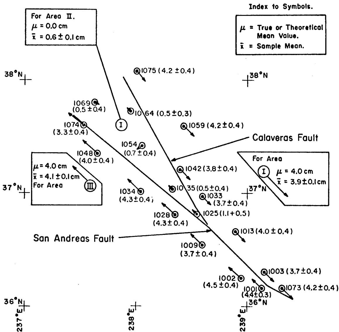
Figure 5-7 Recovery of Velocity Vector (cm), Geometric Mode (250 observations to each station; \sigma_r = 2 cm; Solution Nos. 1-4 and 1-9).
