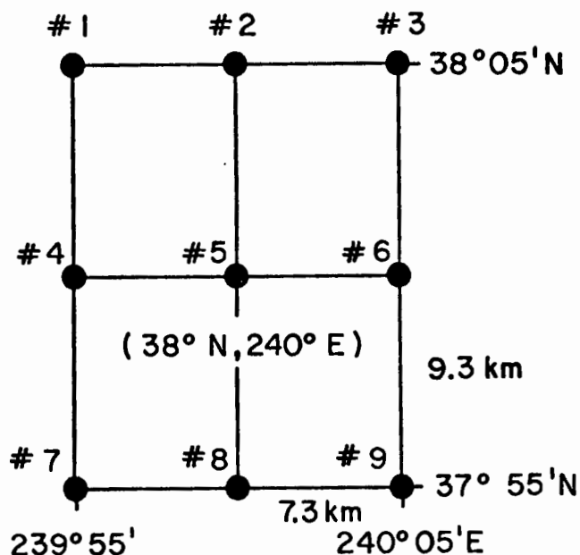
Figure 1-2. Nine-Station Configuration
