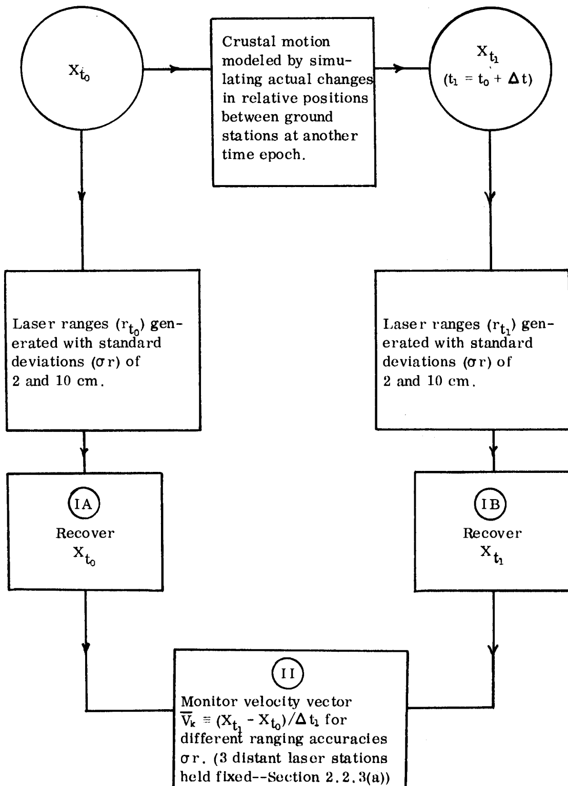
Figure 2-2 Schematic Diagram Showing Recovery of Station Positions and Velocity Vectors
