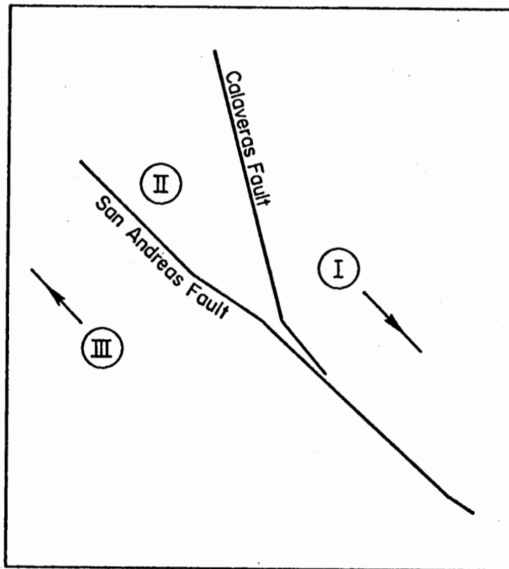
Figure 3-2. Simplified Crustal Motion Pattern
