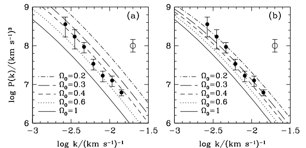
FIG. 1.—Filled circles (with 1 \sigma error bars) show the power spectrum of mass fluctuations at z = 2.5 , derived from Ly \alpha forest spectra by CWPBK. The error bar on the open circle indicates the normalization uncertainty in this measurement: at the 1 \sigma level, all points can be shifted coherently up or down by this amount. Curves show P(k) at z = 2.5 for cluster-normalized models with a power spectrum shape parameter \Gamma = 0.2 and various values of \Omega_M , as indicated. Models with high \Omega_M predict a P(k) that is too low to match the Ly \alpha forest results, and models with low \Omega_M predict a P(k) that is too high. (a) Open models, with \Omega_\Lambda = 0 . (b) Flat models, with \Omega_\Lambda = 1 - \Omega_M .
