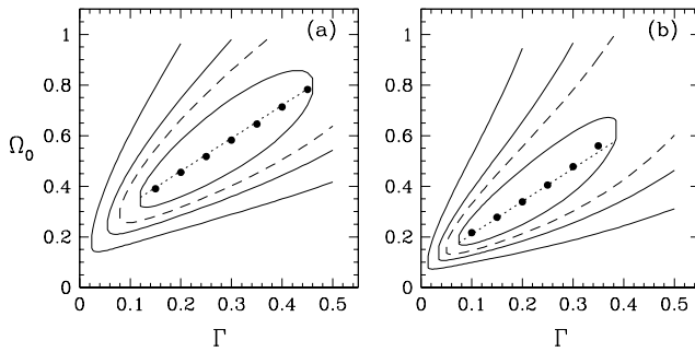
FIG. 2.—Constraints on the parameters of cluster-normalized power spectra, for (a) open models and (b) flat models. Filled circles show the value of \Omega_M that gives the best match (minimum \chi^2 ) to the CWPBK power spectrum parameters at each \Gamma . Dotted lines show the ridgeline eqs. (3). Solid lines show contours of \Delta\chi^2 = 1, 4, 9 in the (\Omega_M, \Gamma) -plane. For a specified value of \Gamma , the intersection of a vertical line with the solid contours gives the 1, 2, and 3 \sigma confidence intervals on \Omega_M . If one ignores external information about \Gamma and considers only the Ly \alpha forest data themselves, then the dashed contour at \Delta\chi^2 = 2.30 represents the 68% confidence constraint on the parameter values.
