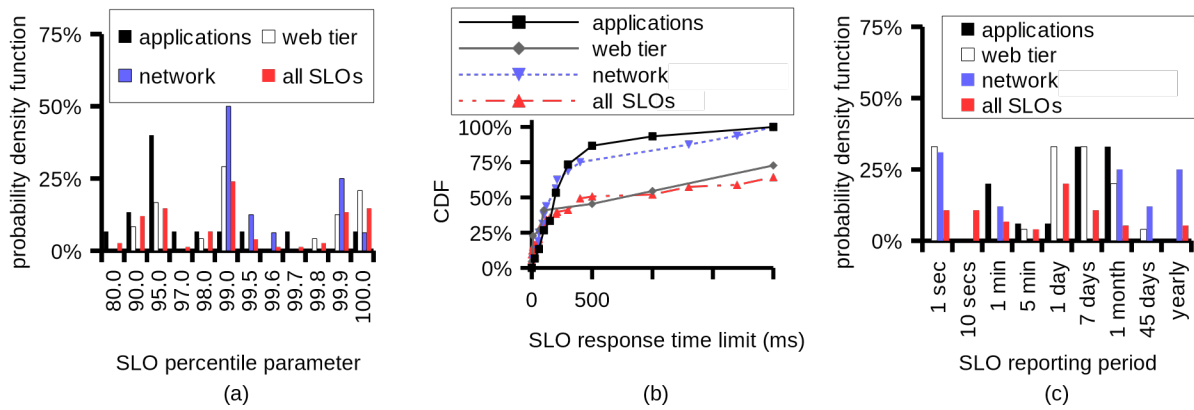
Figure 4. Distributions of (a) SLO percentiles, (b) delay goals and (c) reporting periods. CDF stands for cumulative distribution function
