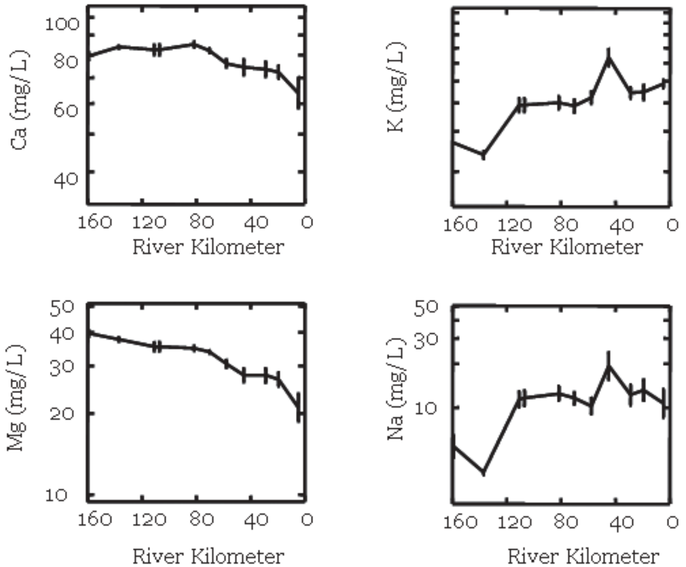
FIGURE 6. Dissolved cations in the Little Miami River during 1996 and 1997. Data are expressed on a logarithmic scale as average concentrations \pm one standard error.
