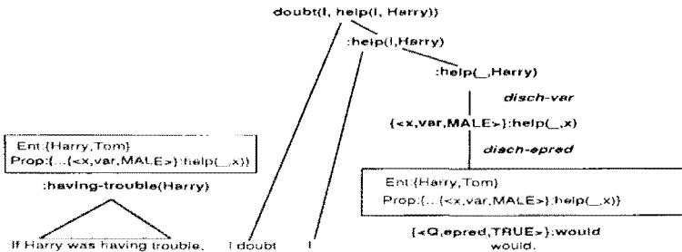
Figure 1: Derivation of Example (6)
