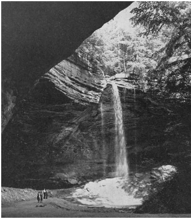
FIGURE 19. View of the upper end of Ash Cave, the waterfall, and the plunge basin below. The firm bedded sandstone forms the projecting cliff. The weaker, cross-bedded sandstone is in the upper part of the reentrant behind the falls. (Ohio Division of Forestry. Photo by Bob Wheaton).
