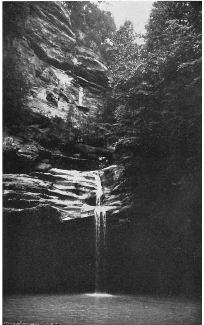
FIGURE 26. The Lower Falls by which Old Man's Creek enters the head of the Lower Gorge. The falls is over only the lower part of the Black Hand sandstone but the entire formation is shown in the valley wall. The plunge basin is probably in the Cuyahoga shale below.
