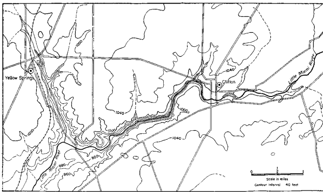
FIGURE 4. Map of the Little Miami River Valley in the Clifton-Yellow Springs region.
