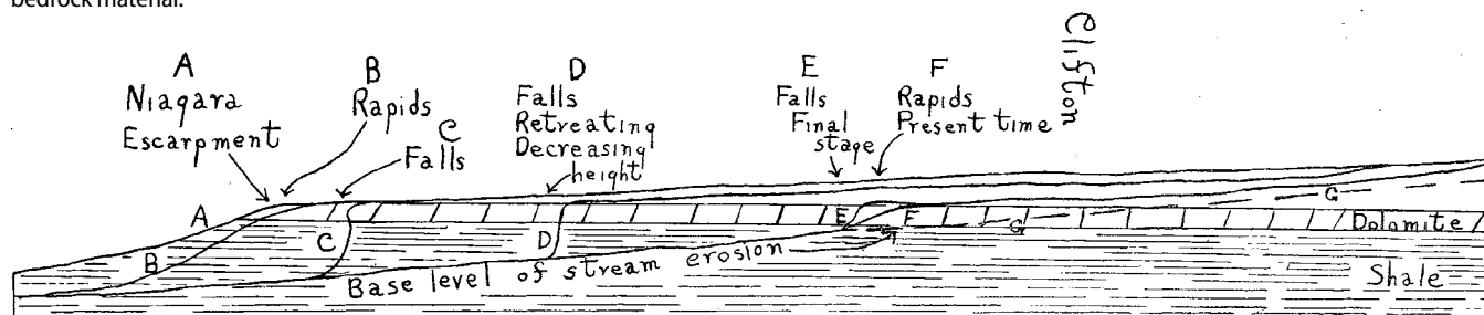
FIGURE 13. Longitudinal section and profile along the Little Miami River showing successive stream profiles during the origin, retreat and disappearance of the falls.
