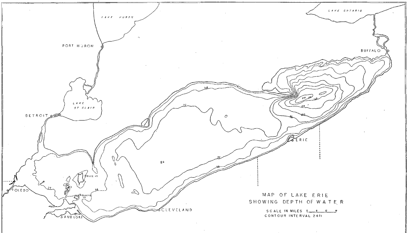
FIGURE 33. Map of Lake Erie showing by contours the depth of the water, which furnishes a basis for a division into eastern, central, and western units.
