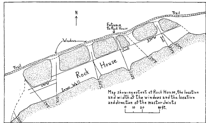
FIGURE 31. Map showing the extent of Rock House, the location and width of the windows, and the location and direction of the master joints.
