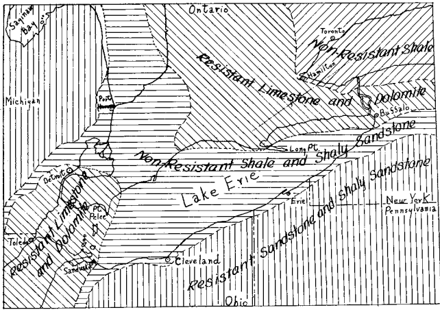
FIGURE 34. Map of the Lake Erie region showing the distribution of the several rock types that have determined the relief features.
