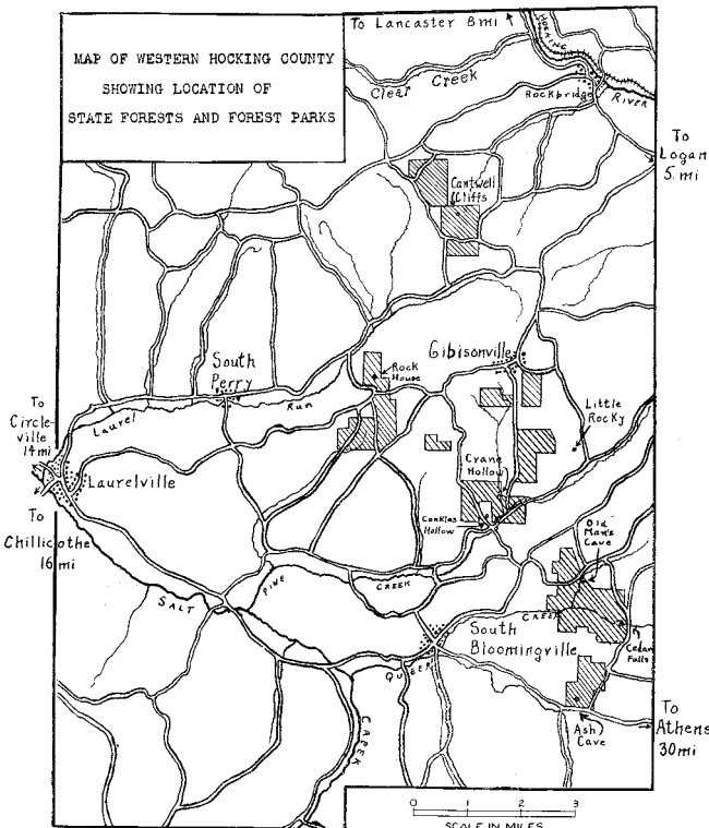
FIGURE 17. Map of western Hocking County showing location of state forests and forest parks.
