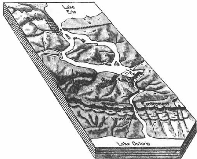
FIGURE 16. JBird's-eye view of Niagara River and Falls, looking south. Greatest length of block, 35 miles. Vertical exaggeration, 2 times. (Reprinted from Outlines of Physical Geology , by Longwell, Knopf, and Flint, published by John Wiley and Sons, Inc.)
