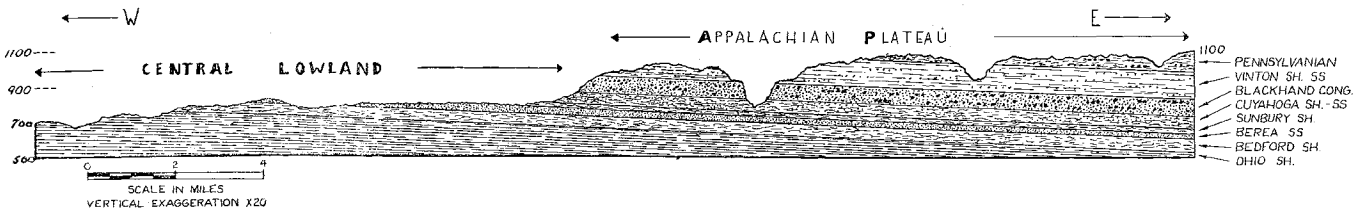
FIGURE 20. West to east cross section of the Appalachian Plateau Front in Hocking County, showing the westward facing escarpment and the slight dip to the east.
