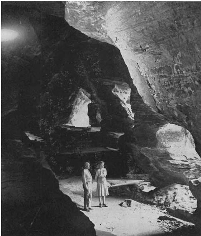
FIGURE 29. Looking southwest along the corridor of Rock House showing the open southwest end and the windows on the right which admit the light. (Ohio Division of Forestry. Photo by Bob Wheaton.)
