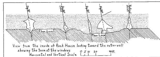
FIGURE 32. View from the inside of Rock House looking toward the outer wall showing the form of the windows, and the position of the cross joints.
