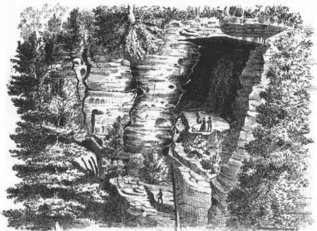
FIGURE 30. The opening at the southwest end of Rock House protected by a rock canopy of the firm upper beds of the Black Hand sandstone. (Geol. Surv. Ohio, Report of Progress in 1870.)
