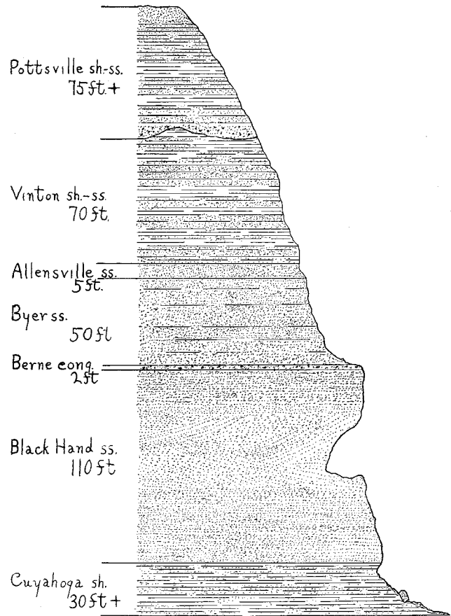
FIGURE 18. Columnar section of the rock formations of Western Hocking County.
