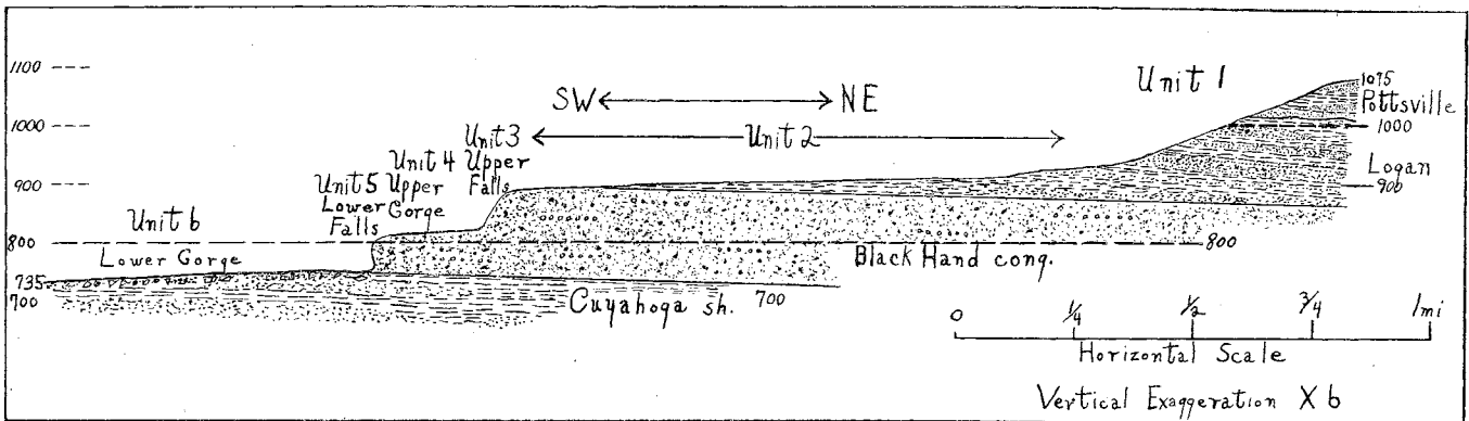
FIGURE 21. Longitudinal section and profile along Old Man's Creek, showing the relation of the several physiographic units to the bedrock materials.
