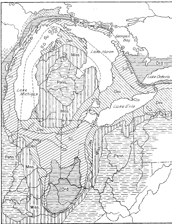
FIGURE 14. Geologic map of the Eastern Interior region showing the distribution of rock systems and the course of the Niagara Escarpment.
