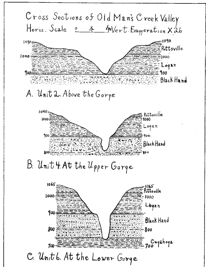
FIGURE 23. Cross sections of Old Man's Creek Valley showing the relation of the form of the valley to the lithology of the rock units.
