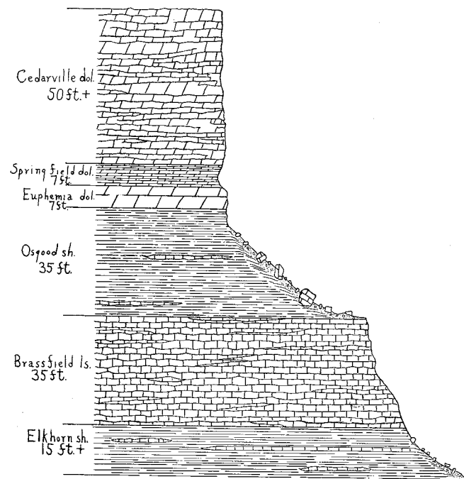
FIGURE 8. Columnar section of the rock formations of the Little Miami River Gorge.
