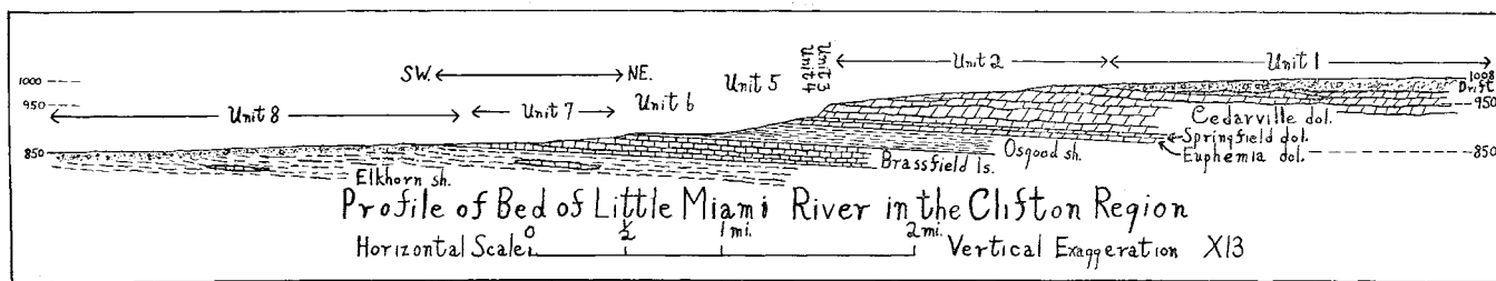
FIGURE 12. Longitudinal section and profile of bed of Little Miami River in the Clifton region, showing the relation of the gradient of the stream to the bedrock material.
