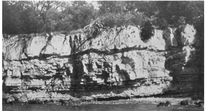
FIGURE 38. Cliff along the south part of the west shore of South Bass Island. The massive brecciated Put-in-Bay dolomite which forms the cliff is being undercut near lake bed in the Tymochtee shaly dolomite.
