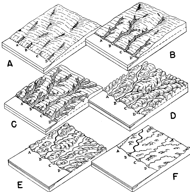
FIGURE 2. Set of block diagrams showing changes in topography during the stream-erosion cycle from youth to old age. (Reprinted by permission from Outlines of Physical Geology , by Longwell, Kropf, and Flint, published by John Wiley and Sons, Inc.)
