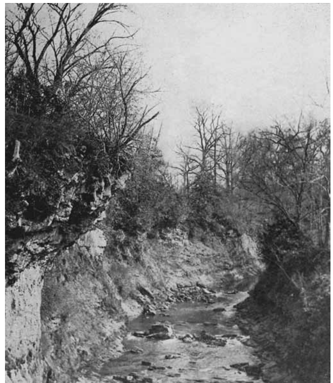
FIGURE 6. The upper part of the Little Miami Gorge just west of Clifton.
