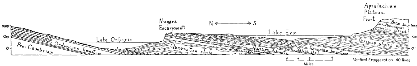
FIGURE 36. North-south section across the Ontario and Erie basins and the adjoining uplands showing the relations of the basins and uplands to the lithology of the rock units.
