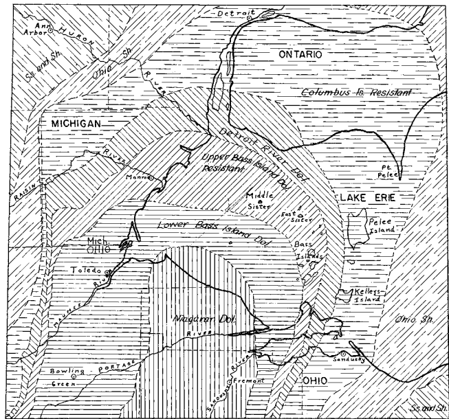
FIGURE 35. Geologic map of the region around the west end of Lake Erie showing the relation of the island belts to the lithology and relative resistance of the rock units.
