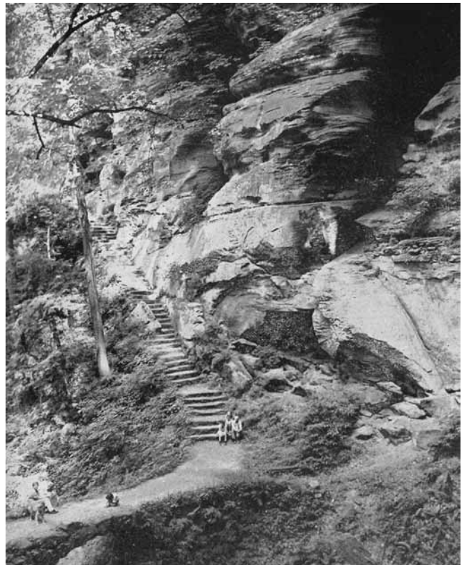
FIGURE 28. The Black Hand sandstone cliff on the face of Rock House. The dark reentrants are the windows leading into Rock House. (Ohio Division of Forestry. Photo by Bob Wheaton).
