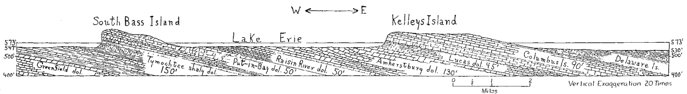
FIGURE 37. East-west section through South Bass and Kelleys islands showing the cuesta form of the islands, the rock units, and the rock structure.
