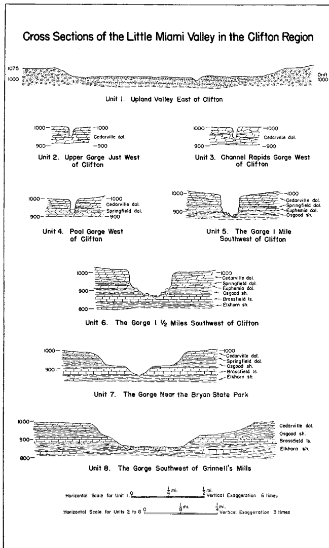
FIGURE 5. Cross sections of the Little Miami River Valley in the Clifton region.
