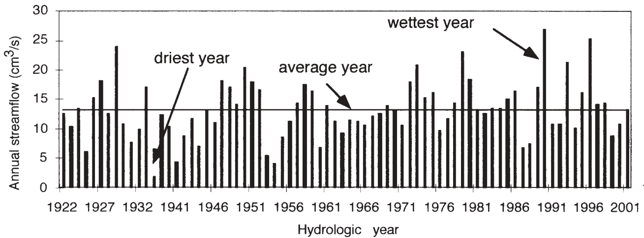
FIGURE 2. Annual streamflow of Big Darby Creek from 1922 to 2002 (USGS station 3230500, Darbyville, OH).
