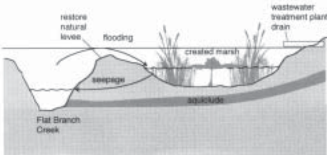
FIGURE 6. Conceptual diagram of riparian wetland creation/restoration at confluence of Flat Branch Creek and Big Darby Creek.
