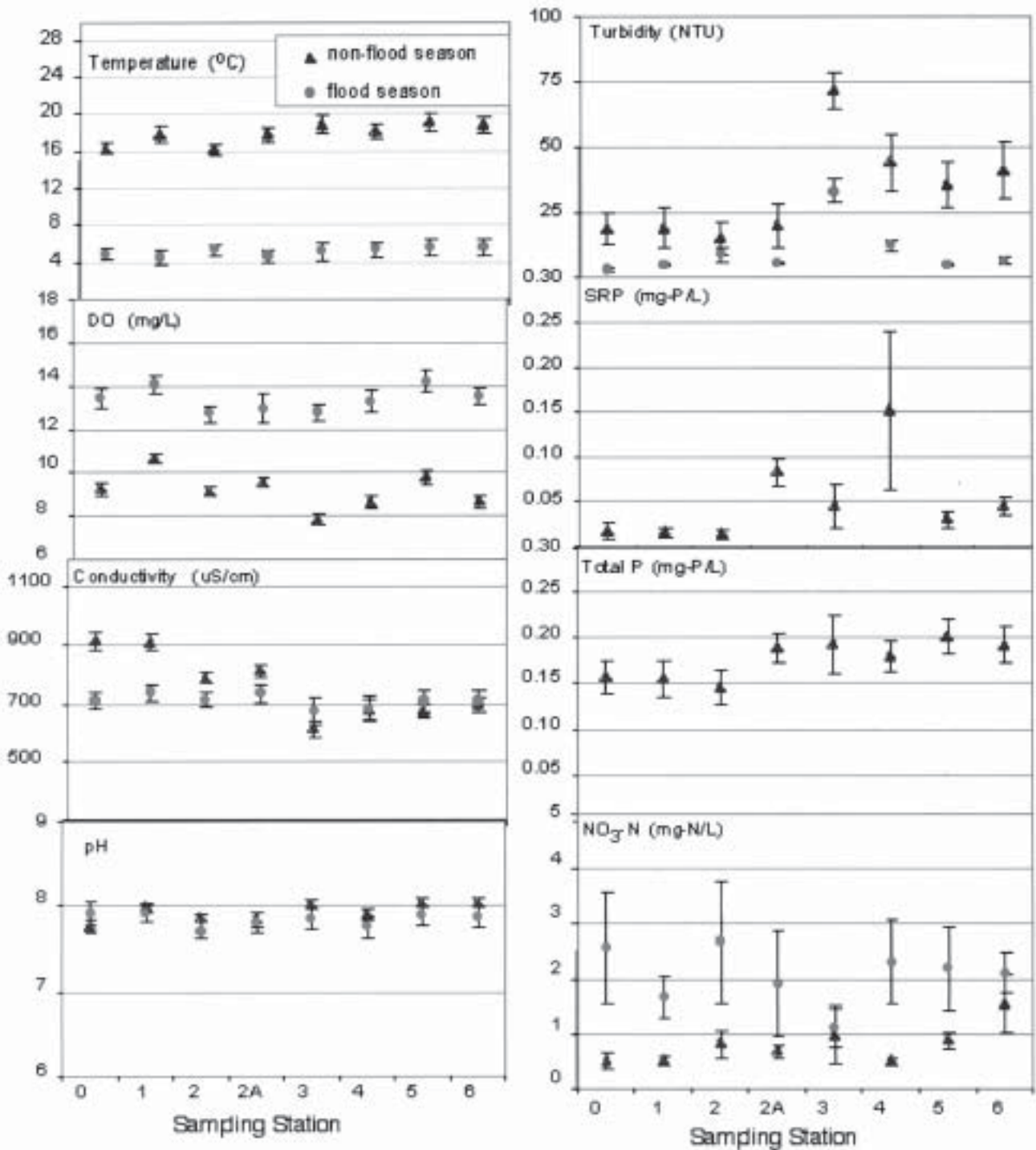
FIGURE 4. Water quality parameters for each monitoring site in Upper Big Darby Creek during the study period. Data are divided into non-growing (flood season) and growing season (non-flood season).
