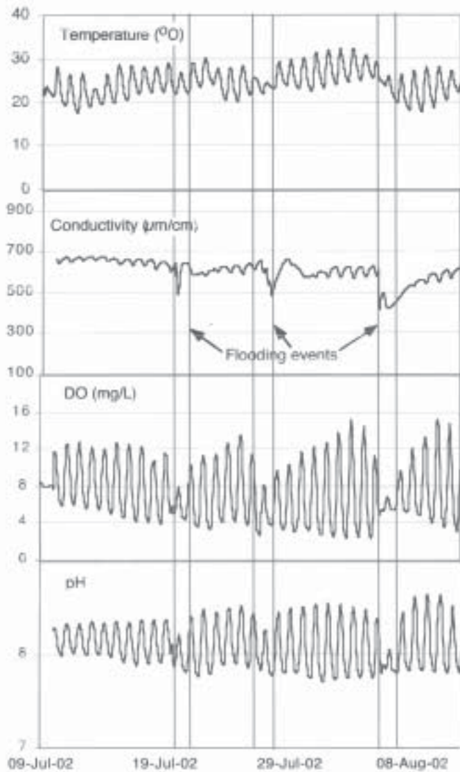
FIGURE 5. Continuous water quality data at Station 5, Big Darby Creek, 9 July – 13 August 2002.
